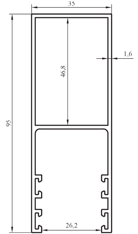
180610 1,236 kg/m
