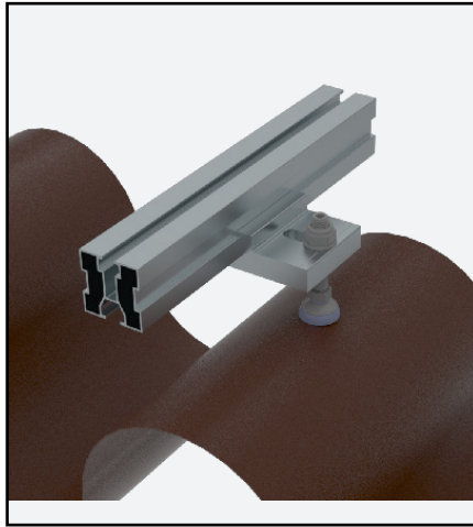
Purlin Connection/ Y-6050
