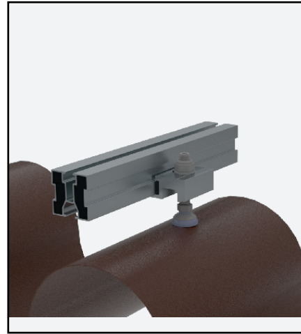
Eco Purlin Connection/ Y-6050E
