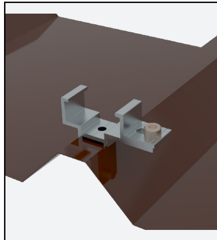
Side Connection / Y-5300
