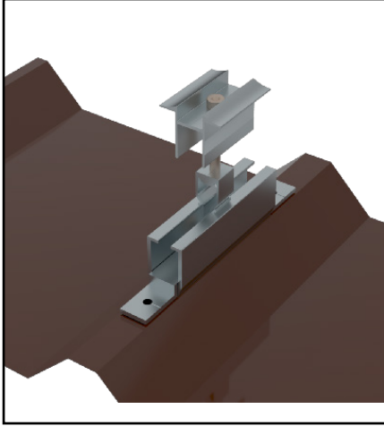
Horizontal Track / Y-5000
