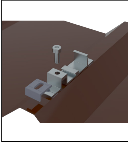
Horizontal Track / Y-5200
